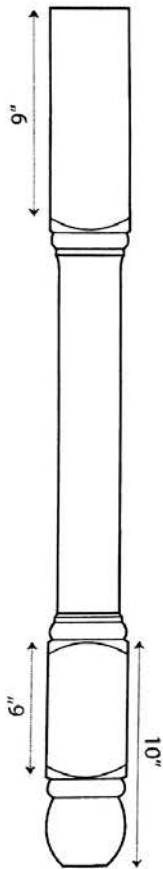
#400-2 3 1/2" x 42"
