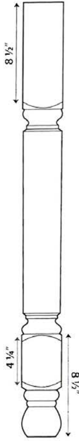
#404 3 1/2" x 36"
