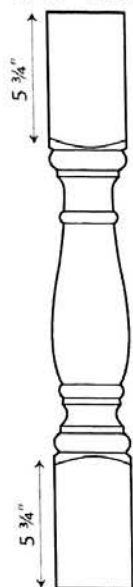
#504-2 3 1/2" x 24"
