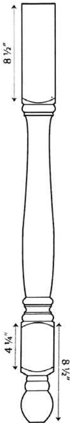
#401-1 3" or 3 1/2" x 36"
