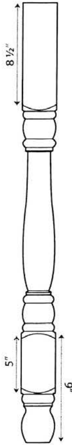
#403 3" x 36"
